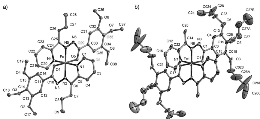
Figure 1. Molecular structure of 1-3 (a) and 4-1 (b) both at 120 K at 50% and 30% probability ellipsoids, respectively. The hydrogen atoms are omitted for clarity.
